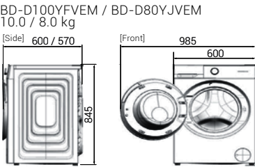
Dimensions (mm)
